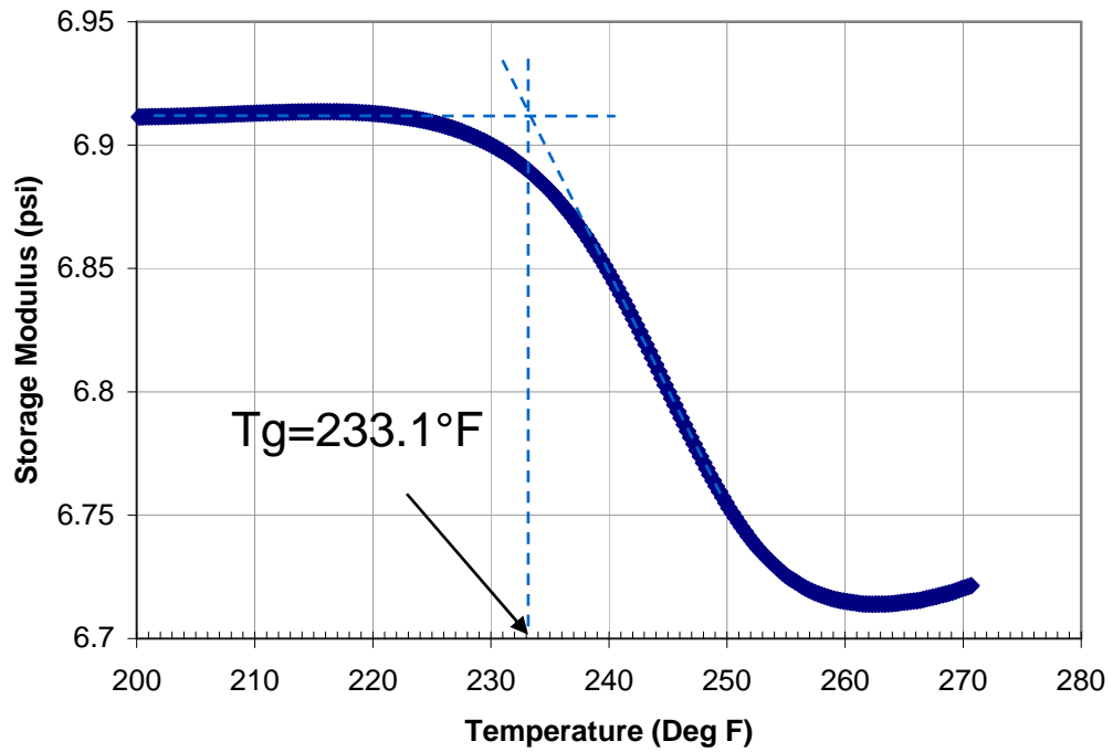
Figure 4.6 Storage modulus vs. temperature from DMA tests of wet T800H/3900-2: (a) DMA-wet1; (b) DMA-wet2.
