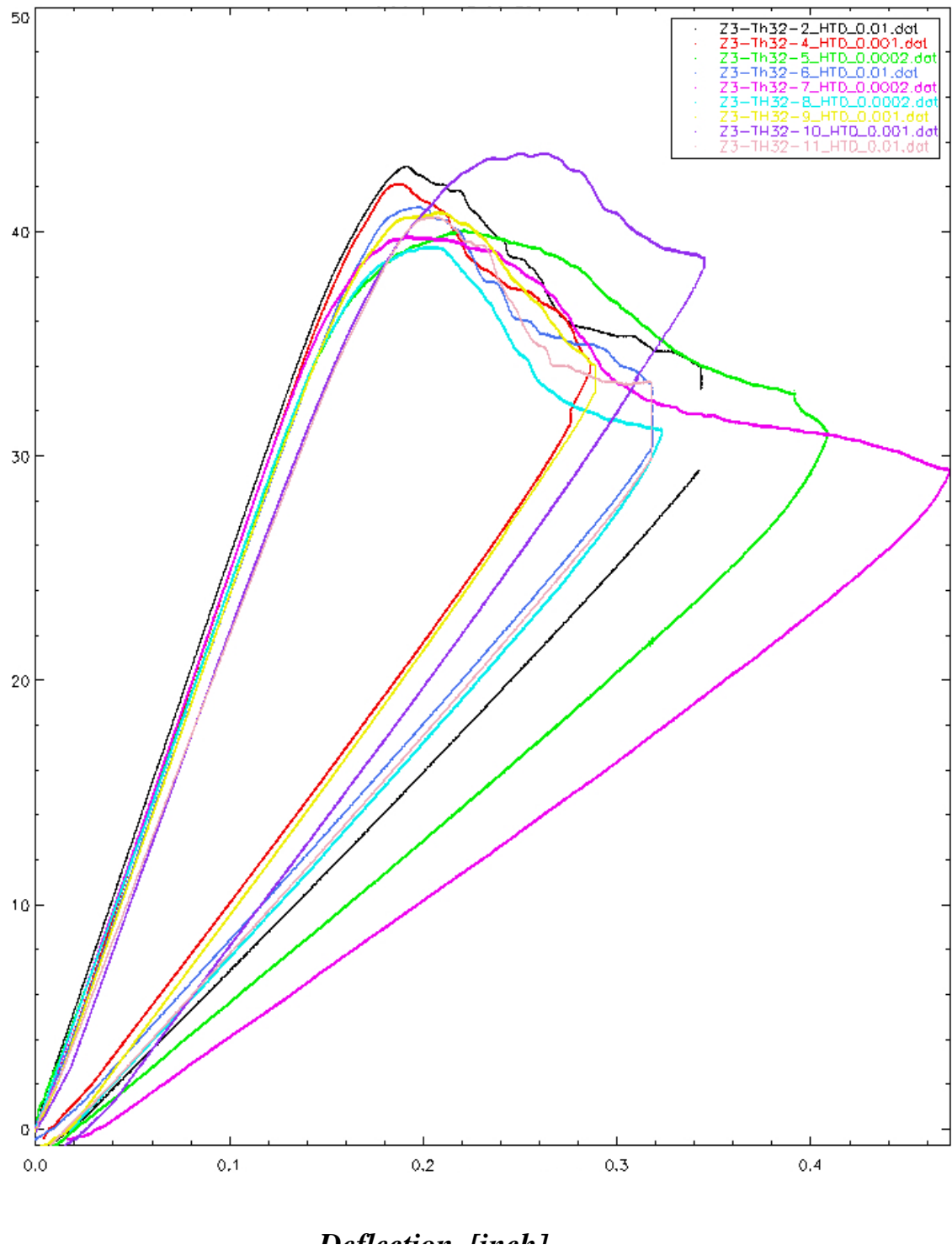
Figure 8.17 Load-deflection curves for 32-ply dry DCB specimens at 125°C.
